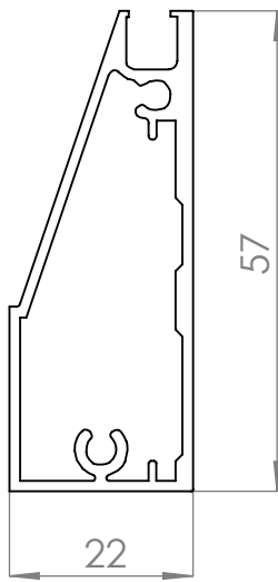
Perfil principal
